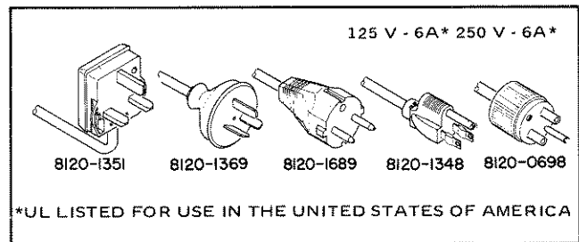
Figure 2-2. Power Cords.
